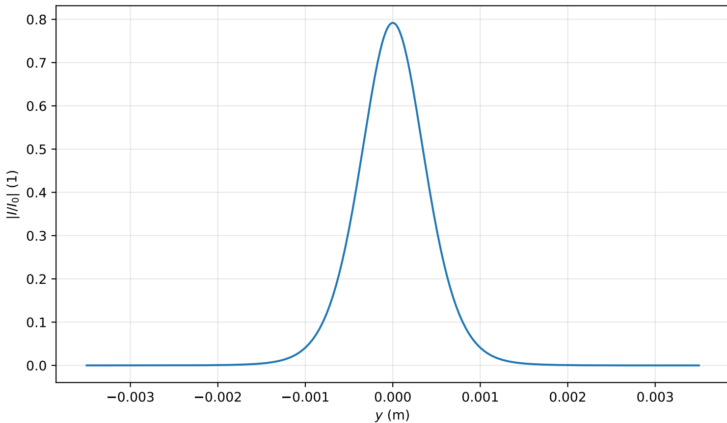
Intensity profile I(x=0, y, z=2.548)/I_0 , \text{Pin}=0.6\text{Pcr} , artificial time
